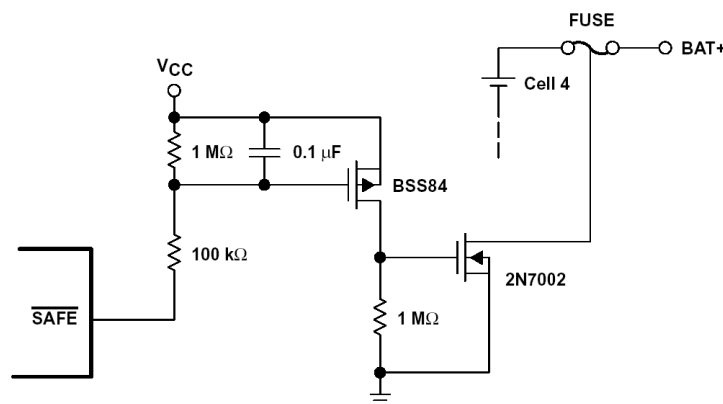
Figure 2. Example SAFE Circuit Implementation
